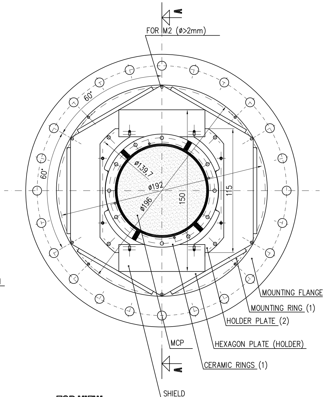
TOP VIEW
